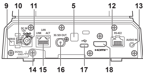
Panel trasero AW-UE40/AW-UE30
